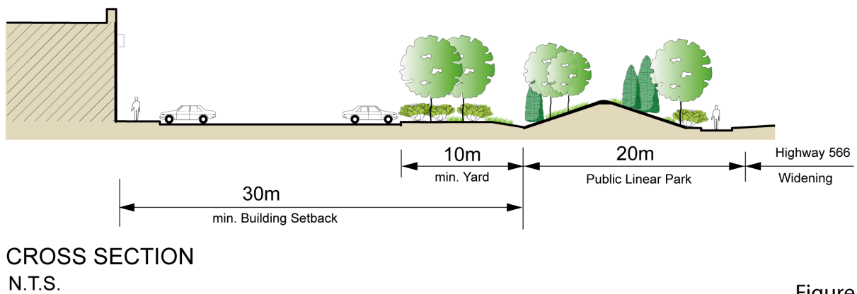
Figure 8 Highway 566 Transition and Park Concept
